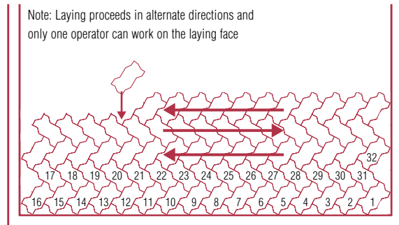
Axis of units not parallel to edge restraints
