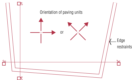
Stringlines used to set out pavement starting point when edge restraints do not suit required orientation of paving units
