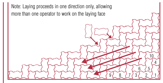
Axis of units parallel to edge restraints
