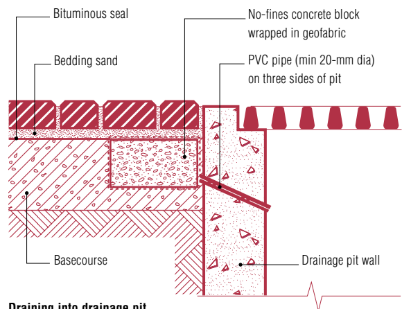
Draining into drainage pit Alternative 2
